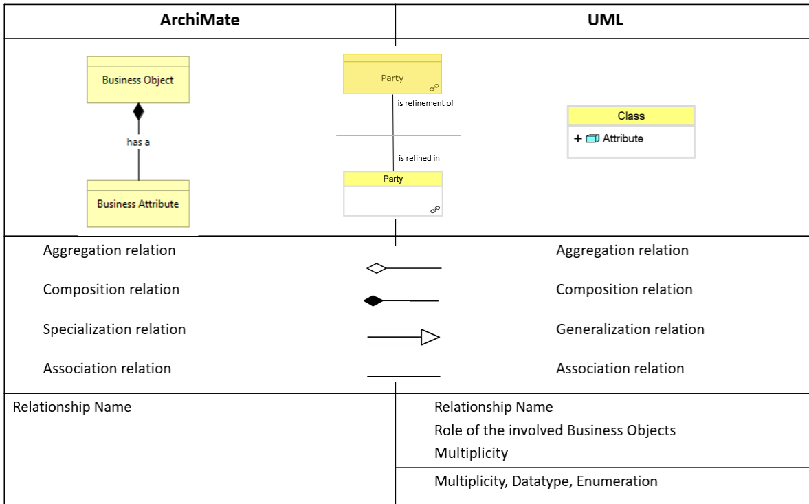
Figure 1 Overview the elements in ArchiMate and UML, used to document data-related deliverables
