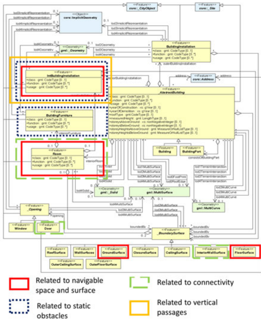
FIGURE 2.1 UML diagram of the building model of CityGML. Names of elements without prefix are defined within the CityGML Building module (LOD4) (from [GKNH12]). The red rectangle refers to classes regarding navigable space and surfaces. The green dashed rectangle indicates a connection among spaces (Room, Door, and InteriorWallSurface). The blue dashed rectangle refers to static obstacles (BuildingFurniture and IntBuildingInstallation). The yellow rectangle represents vertical passages.
